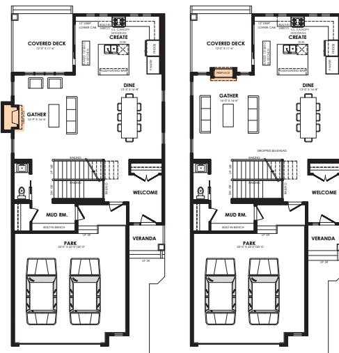
Alternate fireplace location
