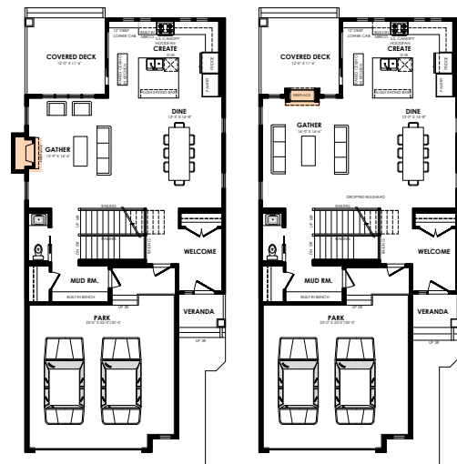
Alternate fireplace location
