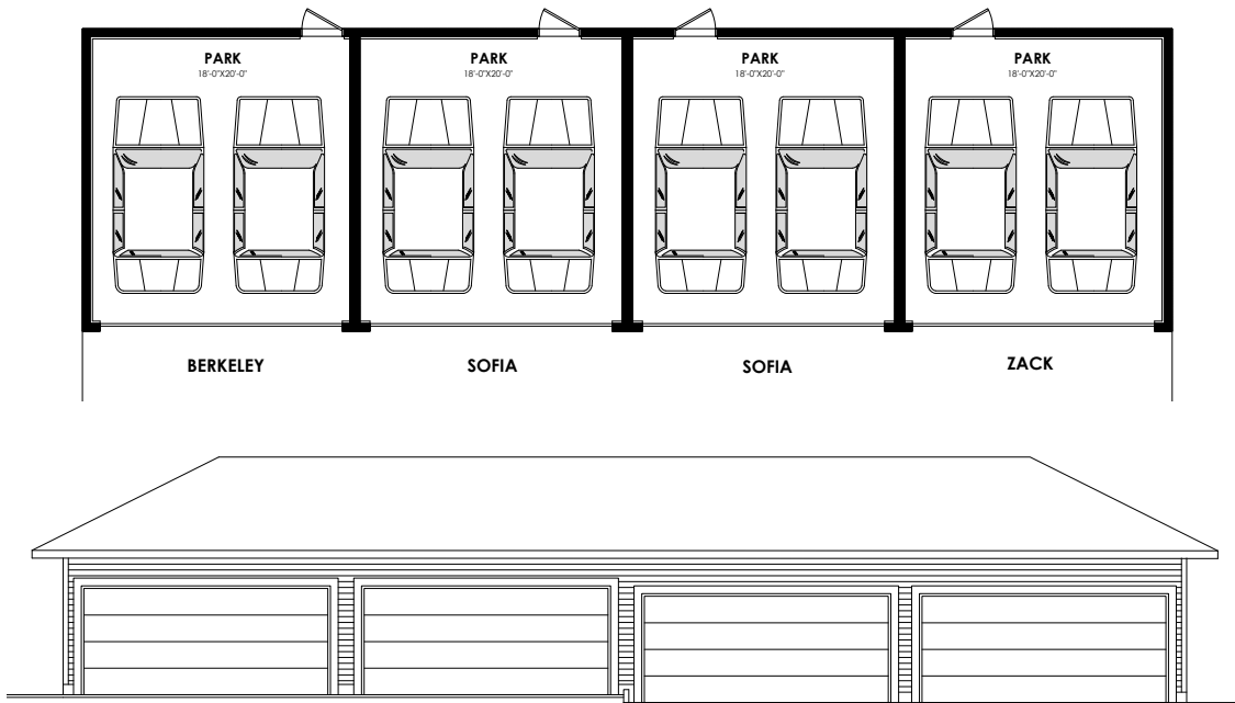
Garage plan
