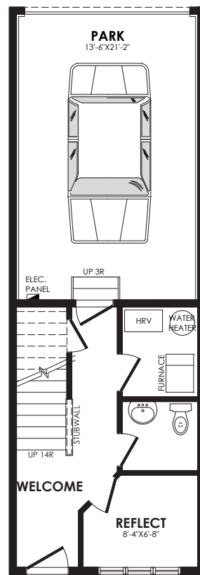
Lower level 537 sq. ft.
